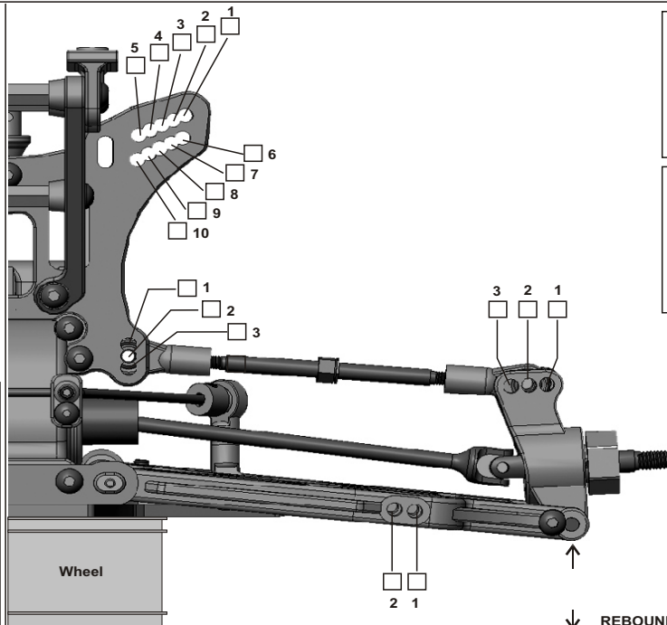
Front Sway Bar Preload
